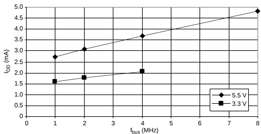
Figure 23-8. Typical Wait Mode I DD with TBM Enabled, LVI Disabled, and PLL Disabled (–40 °C to 85 °C)
