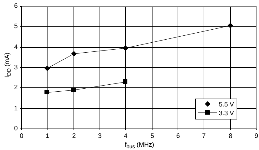
Figure 23-9. Typical Wait Mode I_{DD} , with LVI and TBM Enabled, PLL Disabled ( -40\text{ }^{\circ}\text{C} to 85\text{ }^{\circ}\text{C} )
