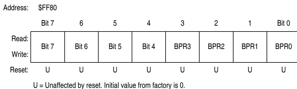
Figure 11-3. FLASH Block Protect Register (FLBPR)
