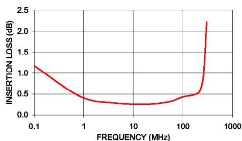
TT4-1A-KK81 INSERTION LOSS
