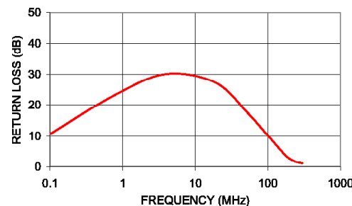
TT4-1A-KK81 INPUT RETURN LOSS
