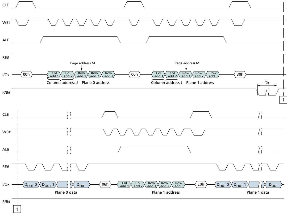
Figure 68: TWO-PLANE PAGE READ
