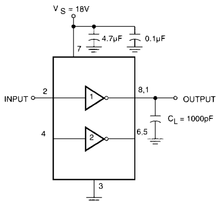
Figure 1. MIC4604/4605 Switching time test circuit.
