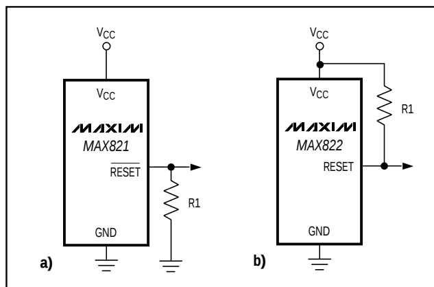
Figure 2. \overline{\text{RESET}}/\text{RESET} Valid to V_{CC} = \text{Ground} Circuit
