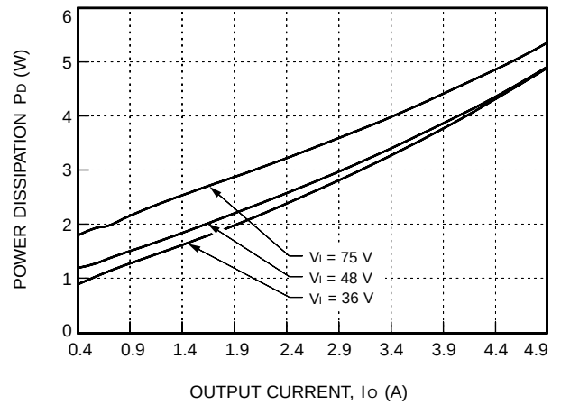
Figure 17. LW025F Power Dissipation vs. Output Current, Ta = 25 °C
