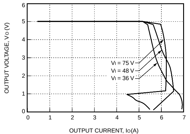
Figure 4. LW025A Typical Output Characteristics
