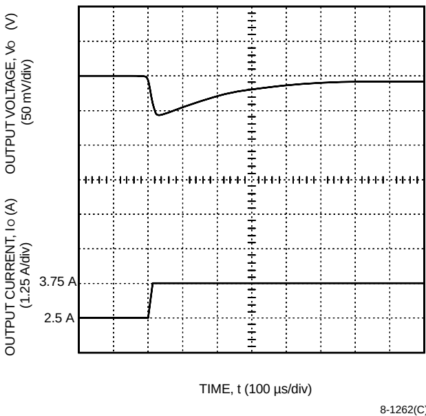
Figure 8. LW025A, F Typical Output Voltage for a Step Load Change from 50% to 75%
