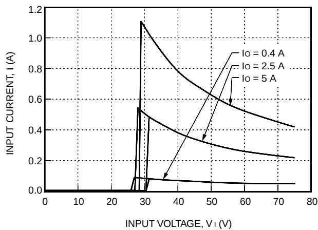
Figure 2. LW025A Typical Input Characteristics
