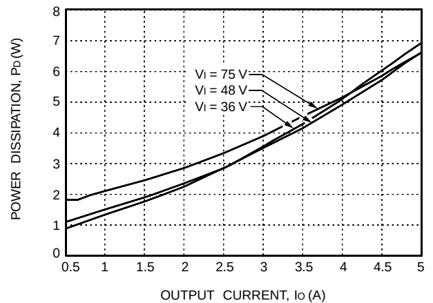
Figure 18. LW025A Power Dissipation vs. Output Current, Ta = 25 °C
