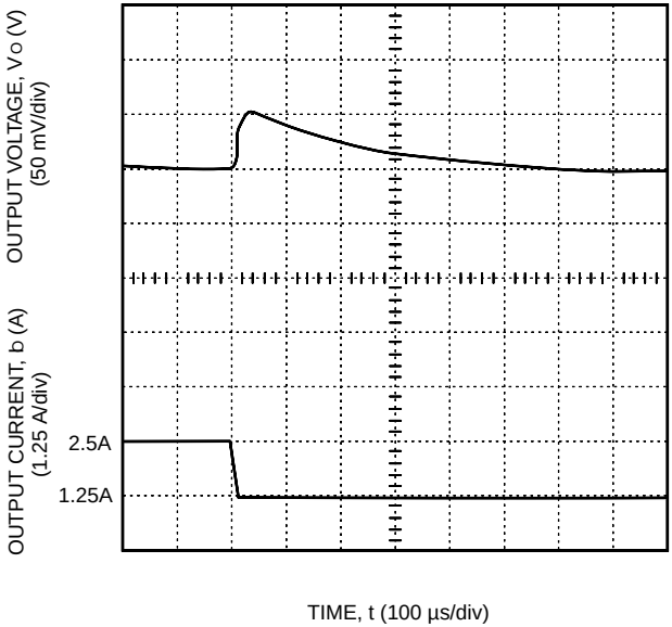
Figure 7. LW025A, F Typical Output Voltage for a Step Load Change from 50% to 25%
