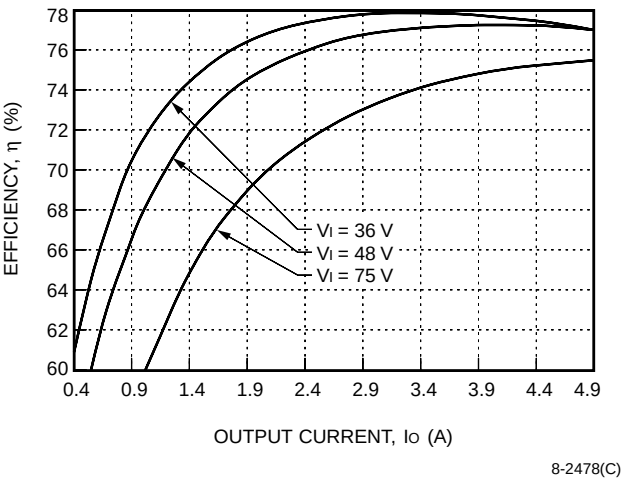
Figure 5. LW025F Typical Converter Efficiency vs. Output Current
