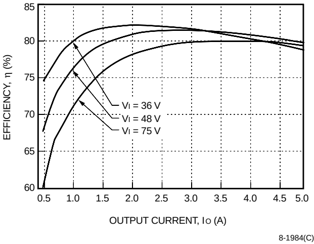
Figure 6. LW025A Typical Converter Efficiency vs. Output Current
