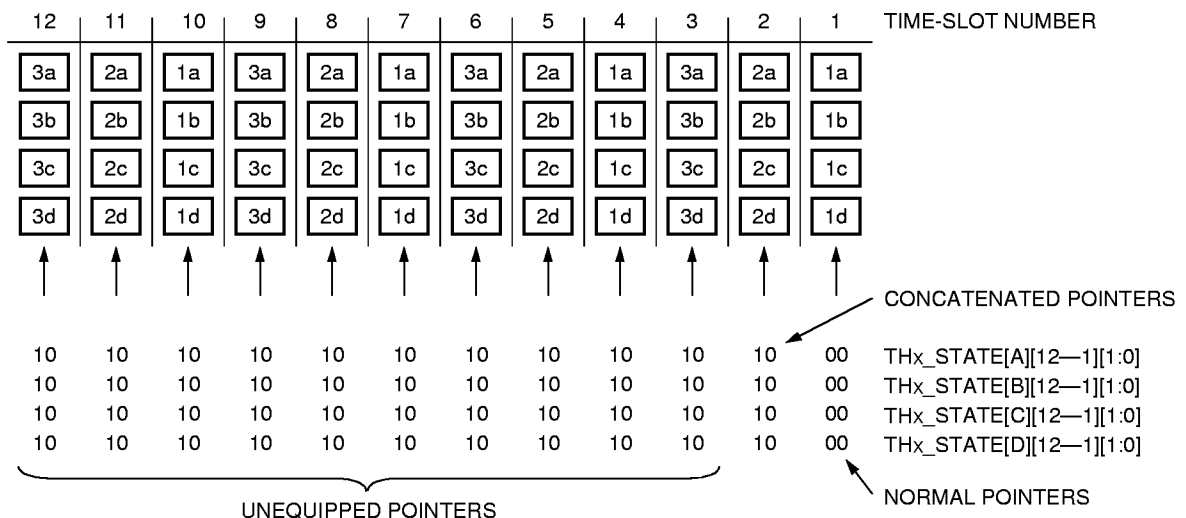
Figure 12. Quad STS-3 Configuration With Each STS-3 Signal Carrying One STS-2c Frame
