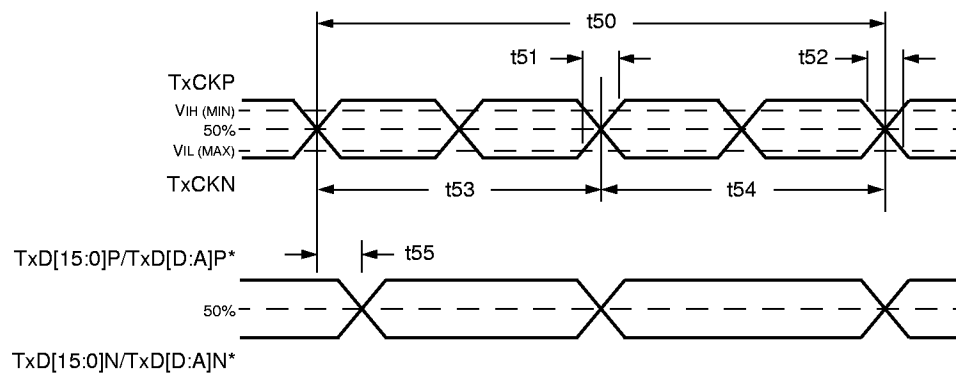
Figure 43. Transmit Line-Side Timing Waveform—STS-48/STM-16 Contraclocking
