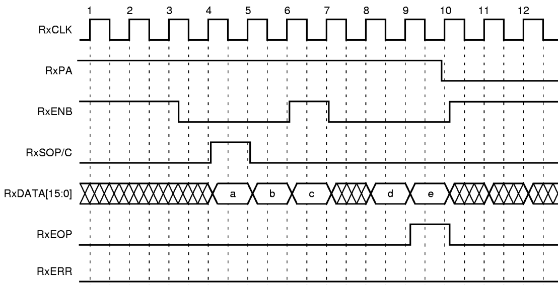
Figure 23. Receive-Side Interface Handshaking in Point-to-Point, Single Cycle Mode
