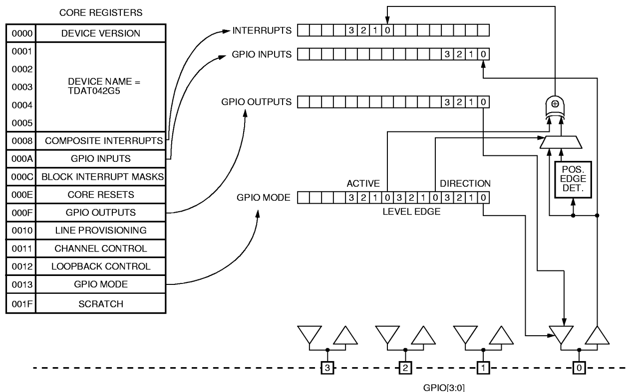
Figure 29. GPIO Functionality
