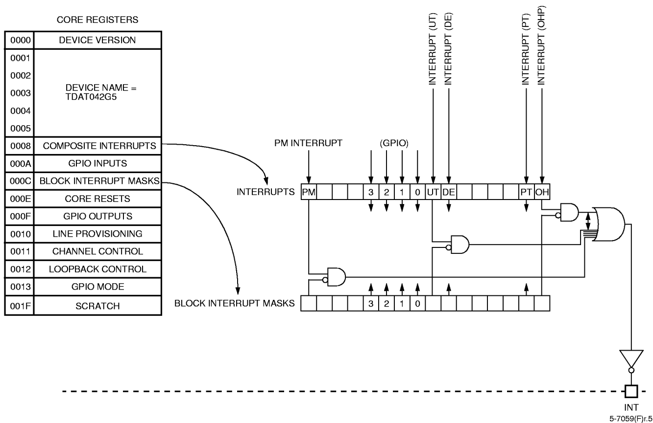
Figure 30. Interrupt Functionality
