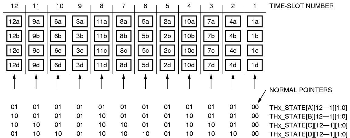
Figure 11. Quad STS-12 Configuration With Each STS-12 Signal Carrying One STS-12c Frame (Channel A), One STS-9c Frame (Channel B), One STS-6c Frame (Channel C), and One STS-3c Frame (Channel D)
