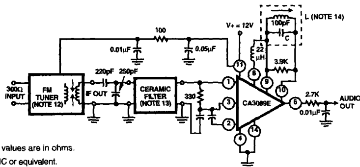
FIGURE 3. TEST CIRCUIT FOR CA3089E USING A SINGLE-TUNED DETECTOR COIL
