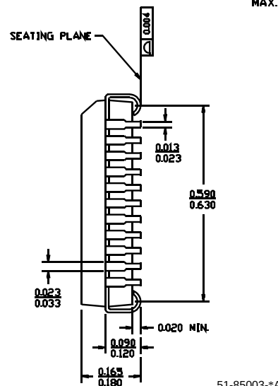
44-Lead Lead(Pb)-Free Plastic Leaded Chip Carrier J67
