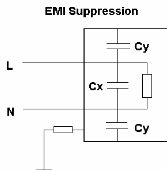
Standard 85/85 X2 circuit
