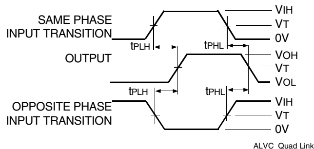
Propagation Delay
