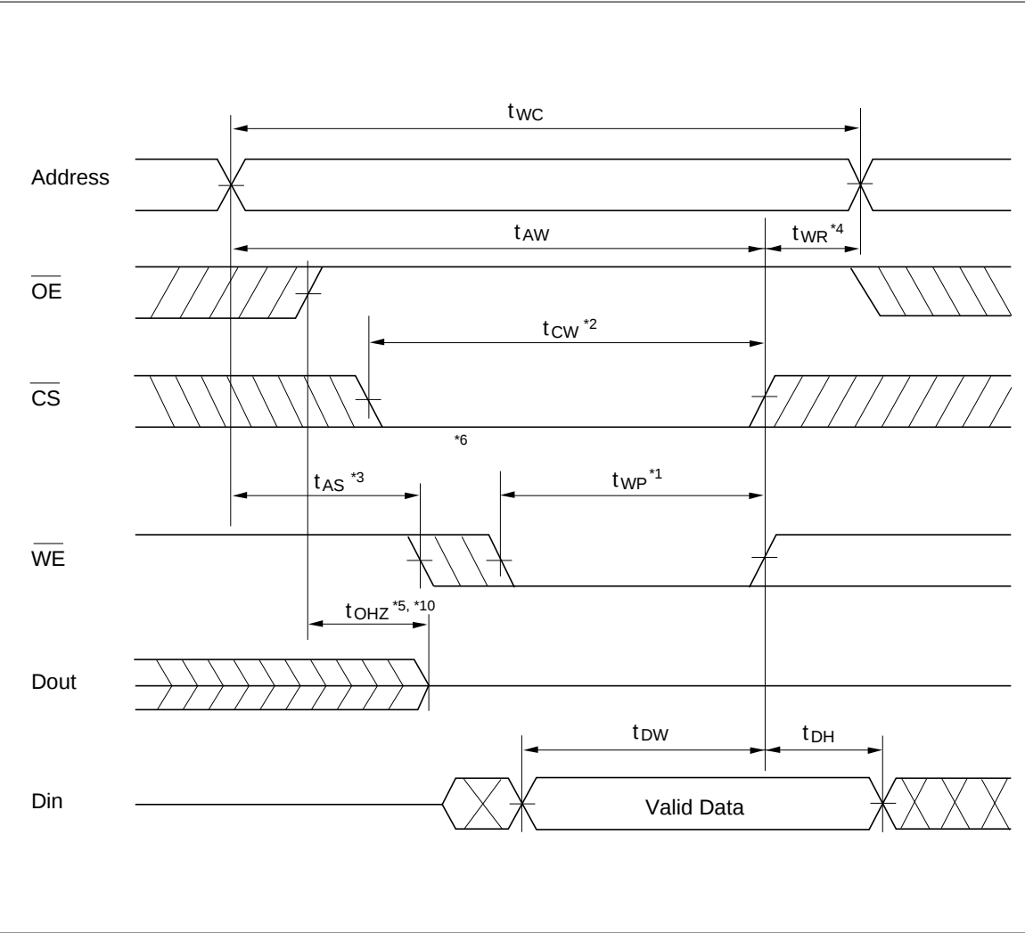
Write Timing Waveform (1) ( \overline{\text{OE}} Clock)
