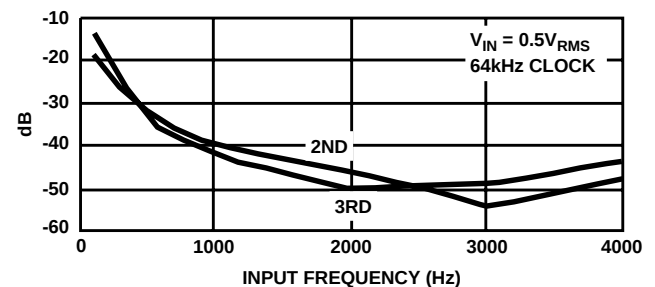
CVSD SIGNAL TO 2ND AND 3RD HARMONIC DISTORTION C-MESSAGE WEIGHTED
