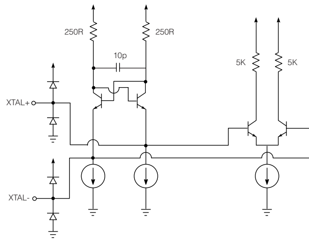
Figure 3-4: Crystal Input
