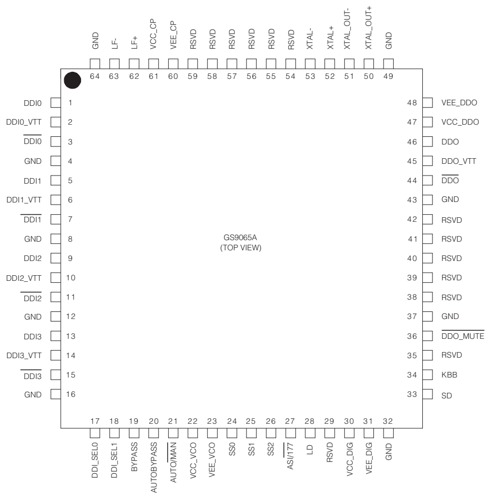
Figure 1-2: 64-Pin LQFP
