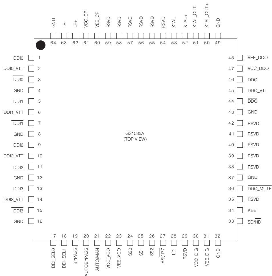
Figure 1-1: 64-Pin LQFP
