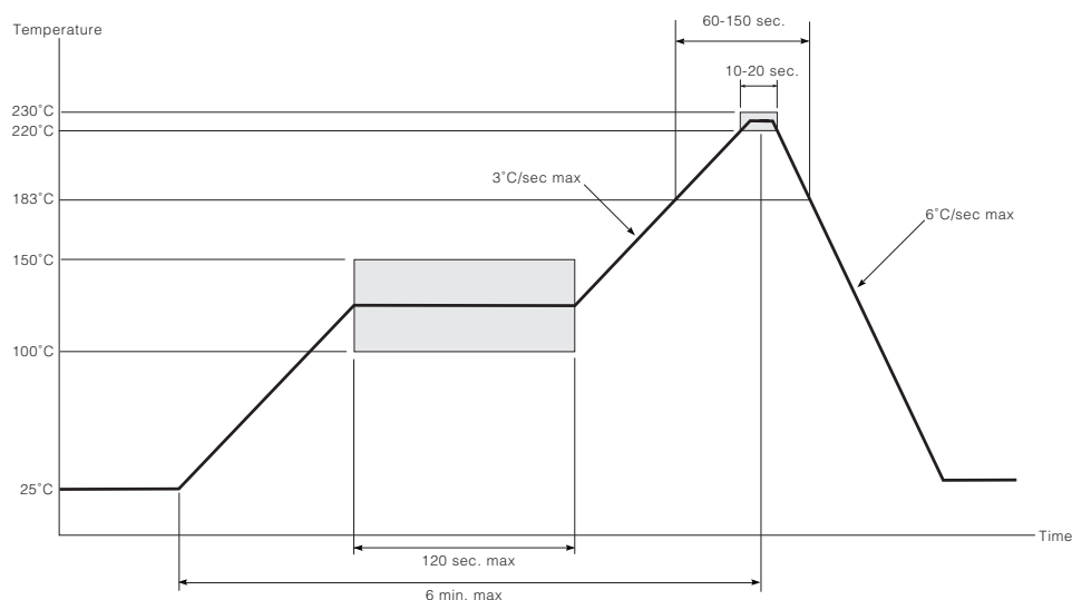
Figure 2-2: Standard Pb Solder Reflow Profile (Pb-free package)
