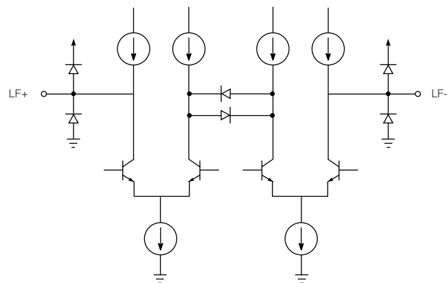
Figure 3-3: Loop Filter
