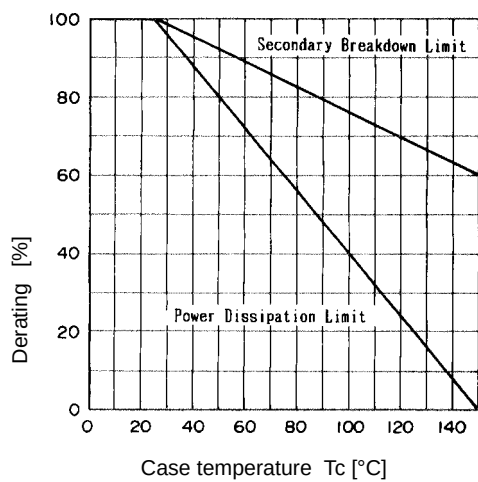
ASO Derating
