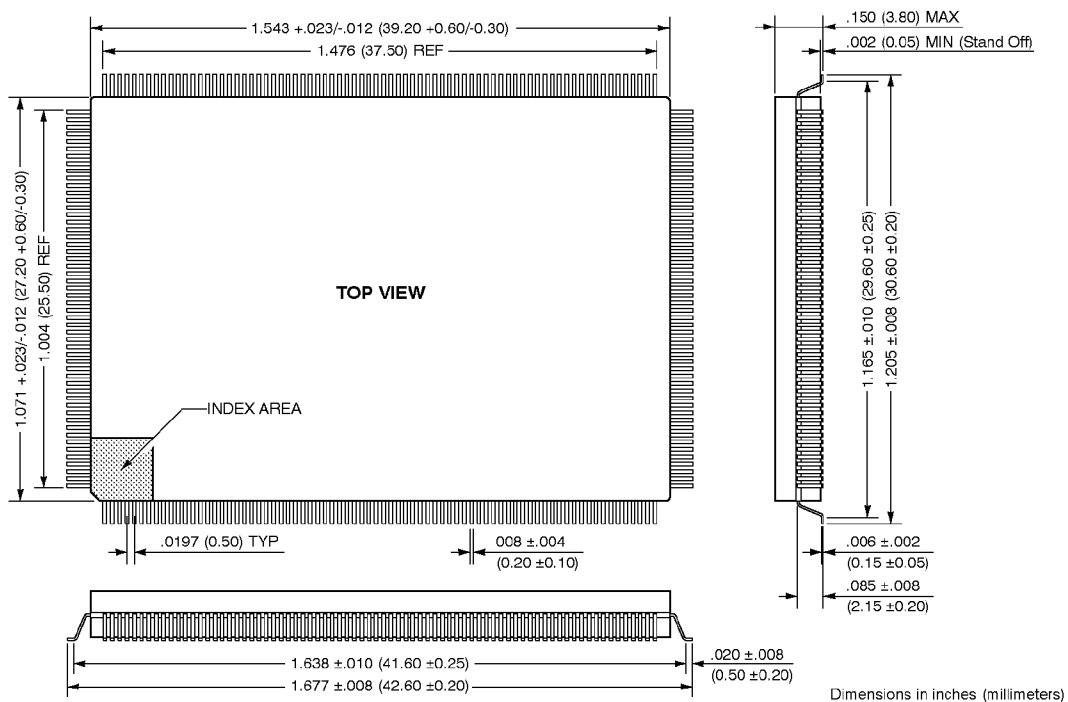
256-LEAD FLAT PACKAGE (CQFP)
