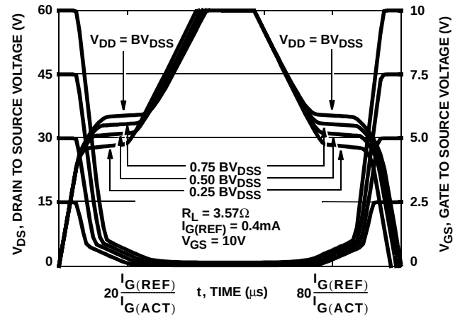
FIGURE 13. NORMALIZED SWITCHING WAVEFORMS FOR CONSTANT CURRENT GATE DRIVE
