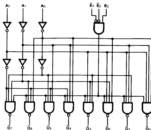
LOGIC DIAGRAM
