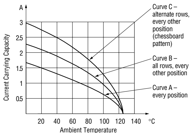
Current Rating For Various Contact Mounting Configurations
