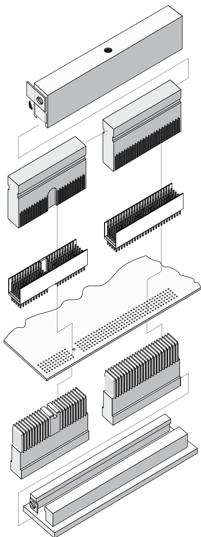
Modular press-fit tool male connector modules 5+2
