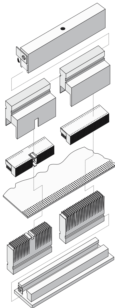
Modular press-fit tool for female connector modules 5+2
