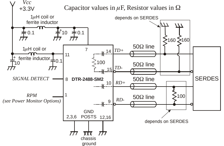
Fig.2 AC-coupled modules
