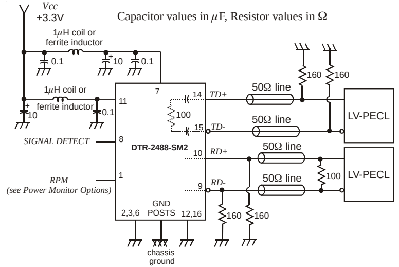
Fig.1 DC-coupled modules
