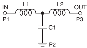
Low pass filter
