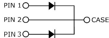
TO-247-3
