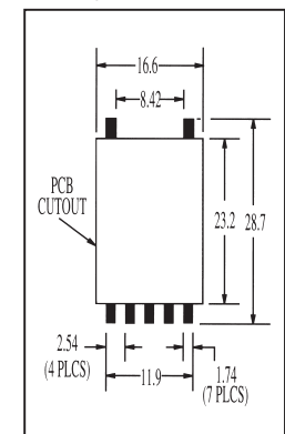
Pad Layout D
