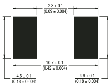
Recommended Pad Layout MF-SM150, 150/33, 200, 250
