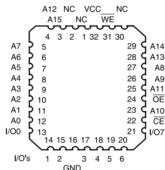
PLCC Top View
