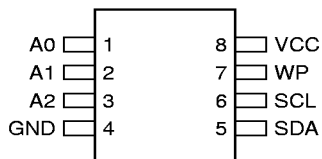
8-Pin SOIC
