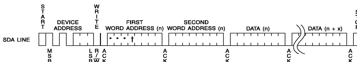
Figure 3. Page Write
