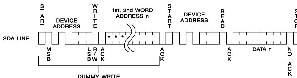
Figure 5. Random Read
