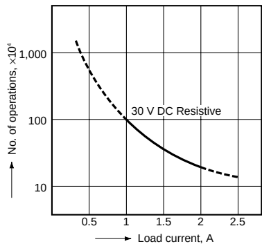
1. Life curve
