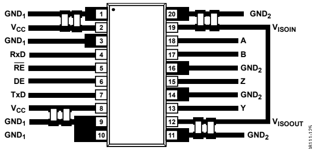
Figure 35. Recommended PCB Layout
