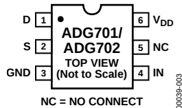
Figure 3. 6-Lead SOT-23
