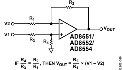
Figure 66. Using the AD855x as a Difference Amplifier
