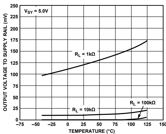
Figure 49. Output Voltage to Supply Rail vs. Temperature
