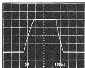
TPC 22. Large-Signal Transient Response
