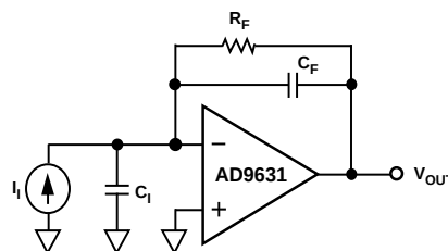
Figure 59. Transimpedance Configuration
