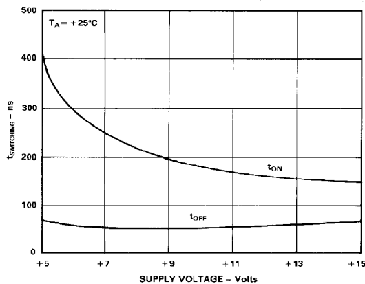
Switching Time vs. Supply Voltage (Single Supply)
