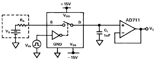
Test Circuit 5. Charge Injection
