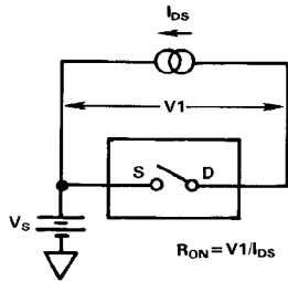
Test Circuit 1
