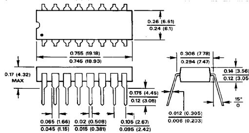
16-Pin Plastic (N-16)
