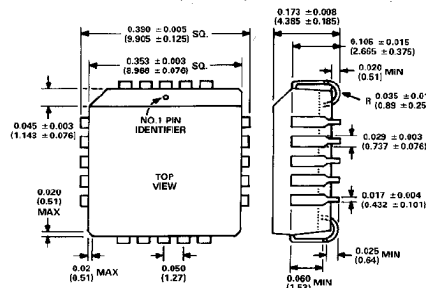
20-Terminal Plastic Leaded Chip Carrier (P-20A)
