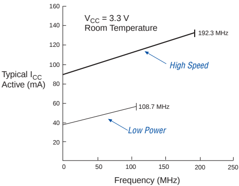
EPM7128A & EPM7128AE
